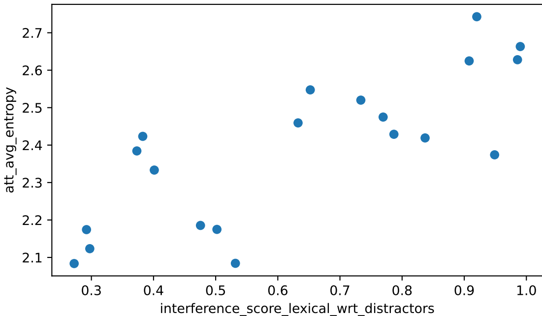
interference_score_lexical_wrt_distractors vs att_avg_entropy Spearman rho=+0.767 (strong), n=20
