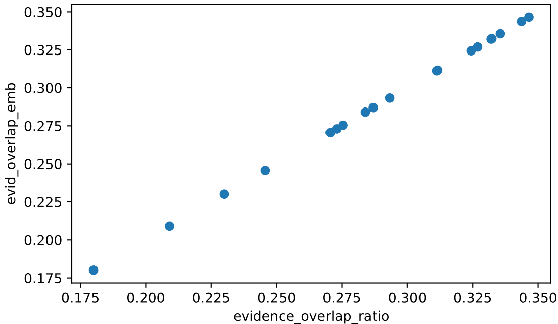
evidence_overlap_ratio vs evid_overlap_emb Spearman rho=+1.000 (strong), n=20
