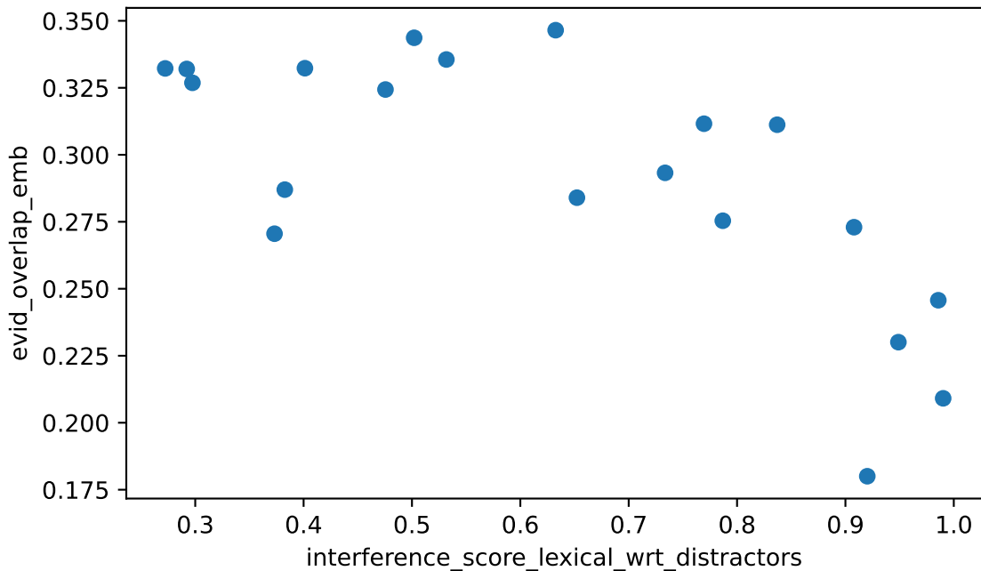
interference_score_lexical_wrt_distractors vs evid_overlap_emb Spearman rho=-0.654 (moderate), n=20
