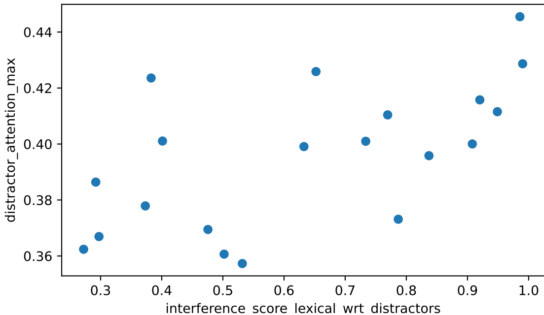
interference_score_lexical_wrt_distractors vs distractor_attention_max Spearman rho=+0.598 (moderate), n=20
