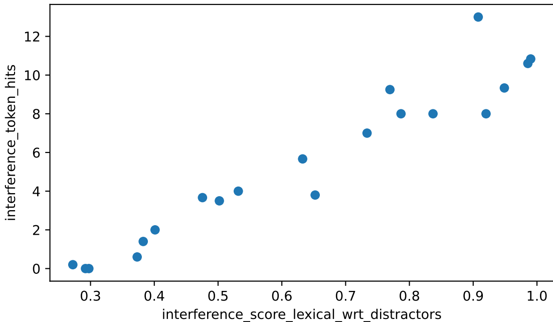
interference_score_lexical_wrt_distractors vs interference_token_hits Spearman rho=+0.960 (strong), n=20
