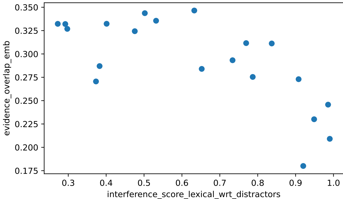
interference_score_lexical_wrt_distractors vs evidence_overlap_emb Spearman rho=-0.654 (moderate), n=20
