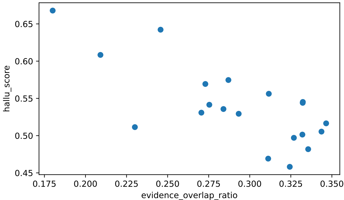
evidence_overlap_ratio vs hallu_score Spearman rho=-0.558 (moderate), n=20
