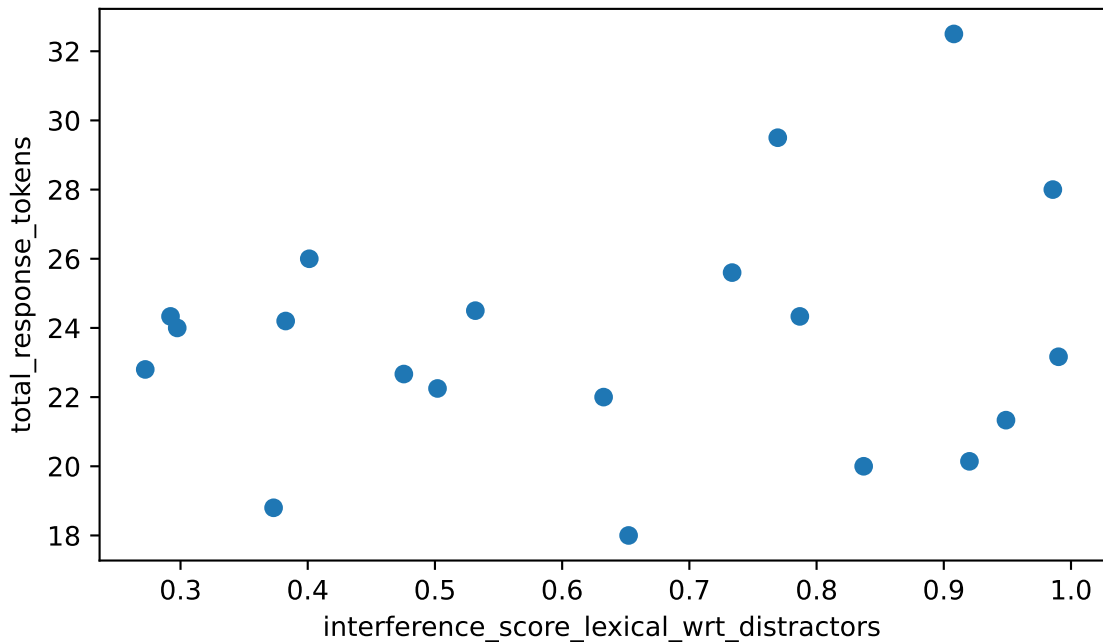
interference_score_lexical_wrt_distractors vs total_response_tokens Spearman rho=+0.068 (weak), n=20
