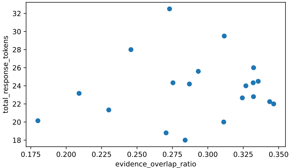
evidence_overlap_ratio vs total_response_tokens Spearman \rho =+0.126 (weak), n=20
