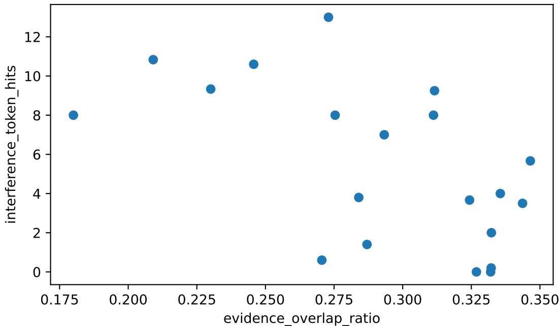
evidence_overlap_ratio vs interference_token_hits Spearman rho=-0.570 (moderate), n=20
