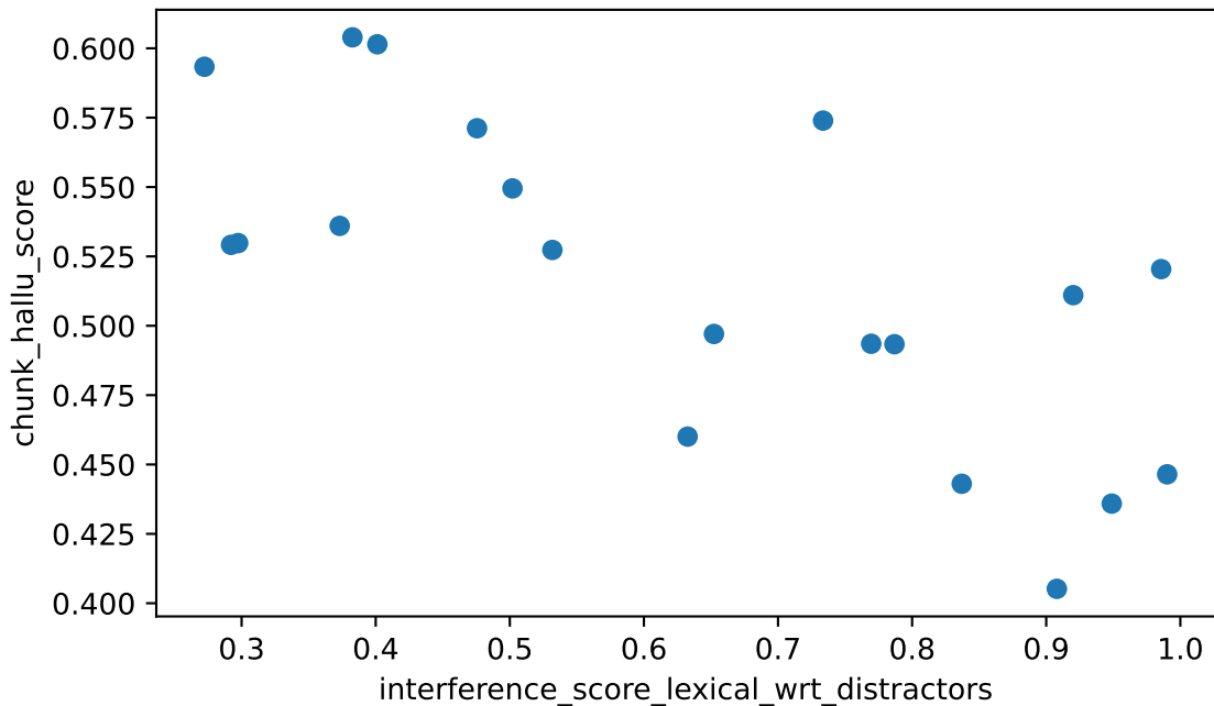
interference_score_lexical_wrt_distractors vs chunk_hallu_score Spearman rho=-0.731 (strong), n=20
