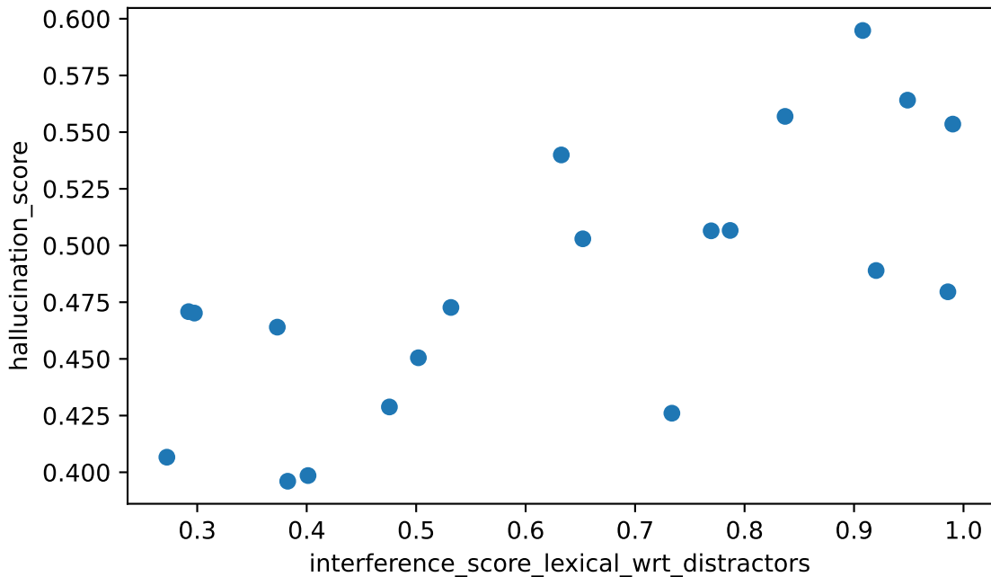
interference_score_lexical_wrt_distractors vs hallucination_score Spearman rho=+0.731 (strong), n=20
