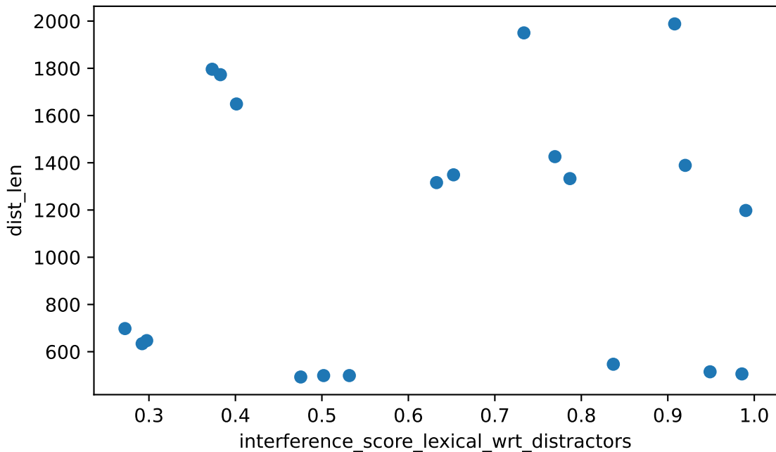
interference_score_lexical_wrt_distractors vs dist_len Spearman rho=+0.004 (weak), n=20
