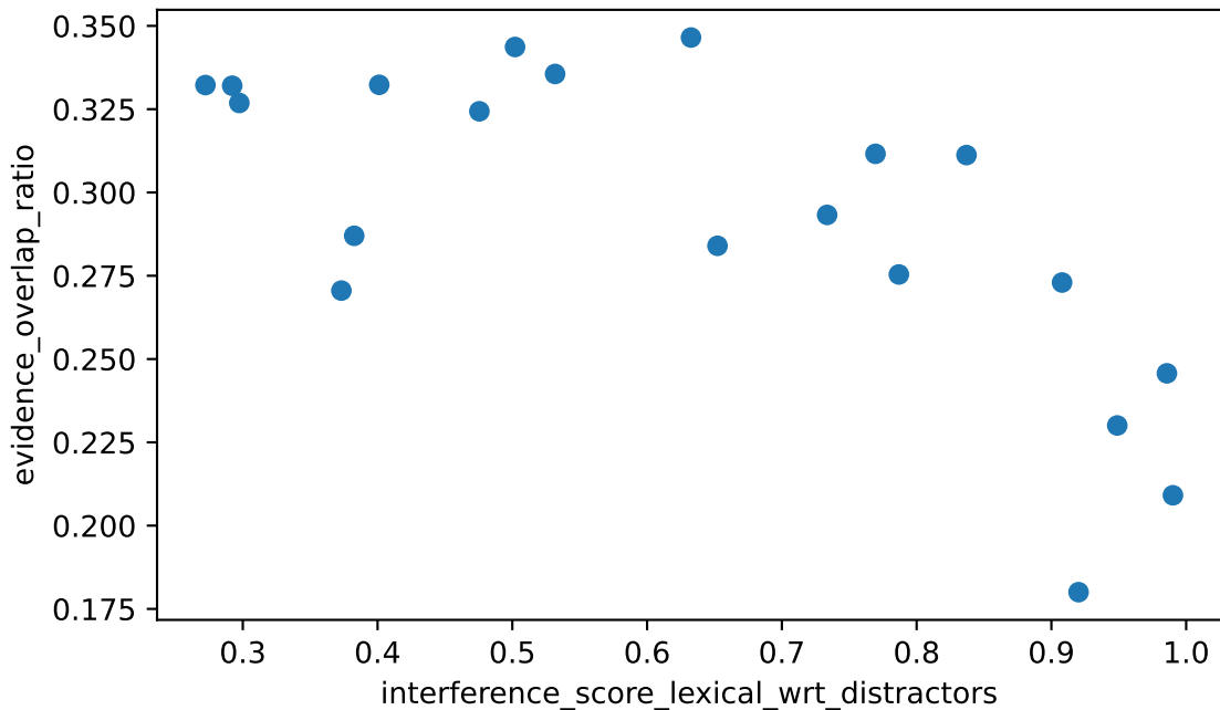
interference_score_lexical_wrt_distractors vs evidence_overlap_ratio Spearman rho=-0.654 (moderate), n=20
