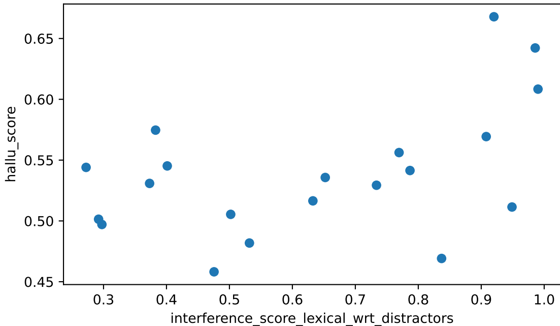
interference_score_lexical_wrt_distractors vs hallu_score Spearman rho=+0.400 (weak), n=20
